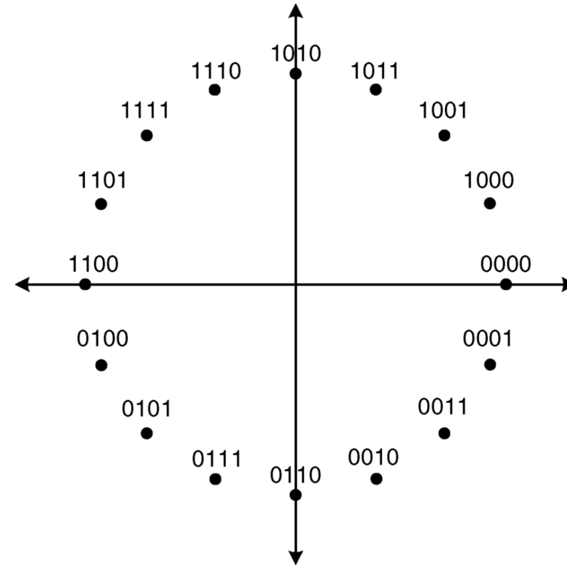
(b) 16PSK 14,000 bps Modem
